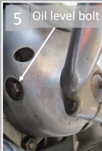
Norton Commando: How to change the gearbox oil
